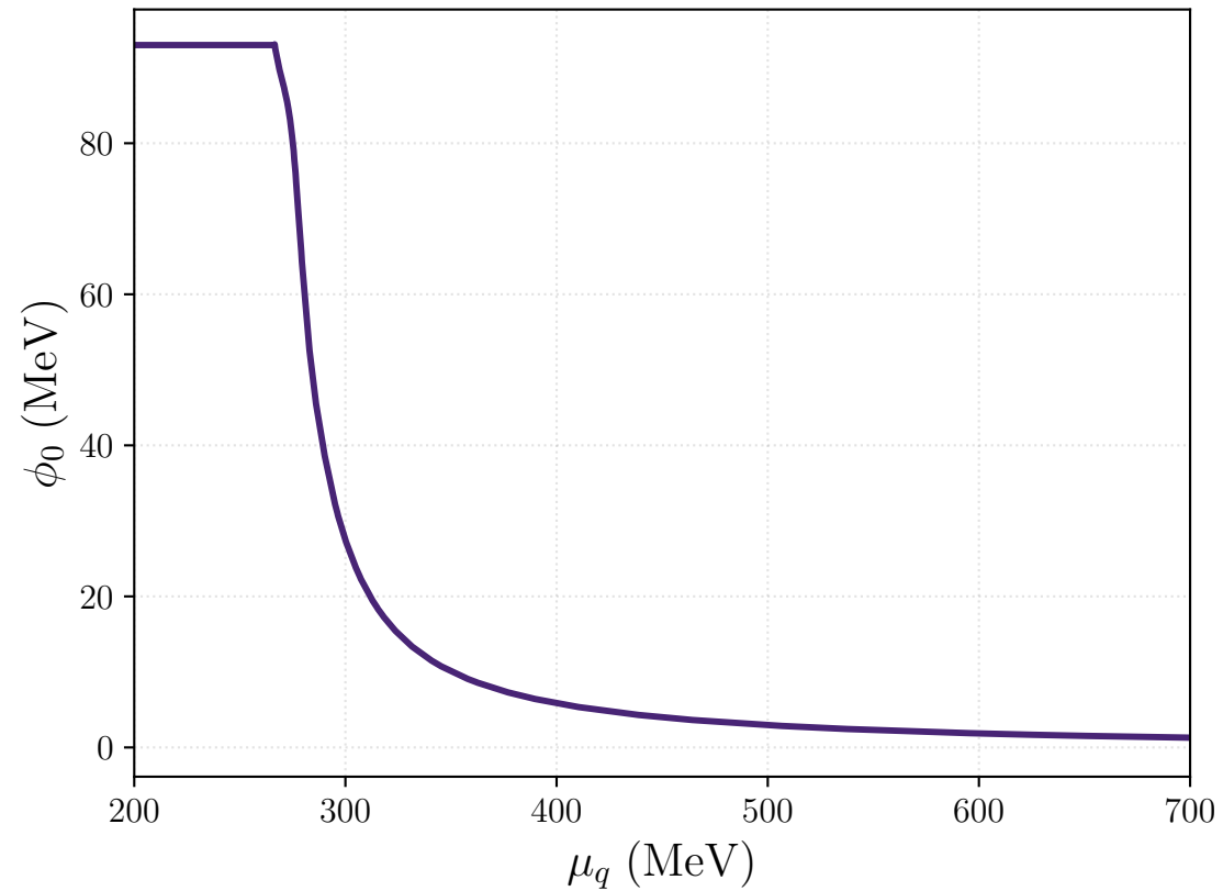
Chiral condensate
