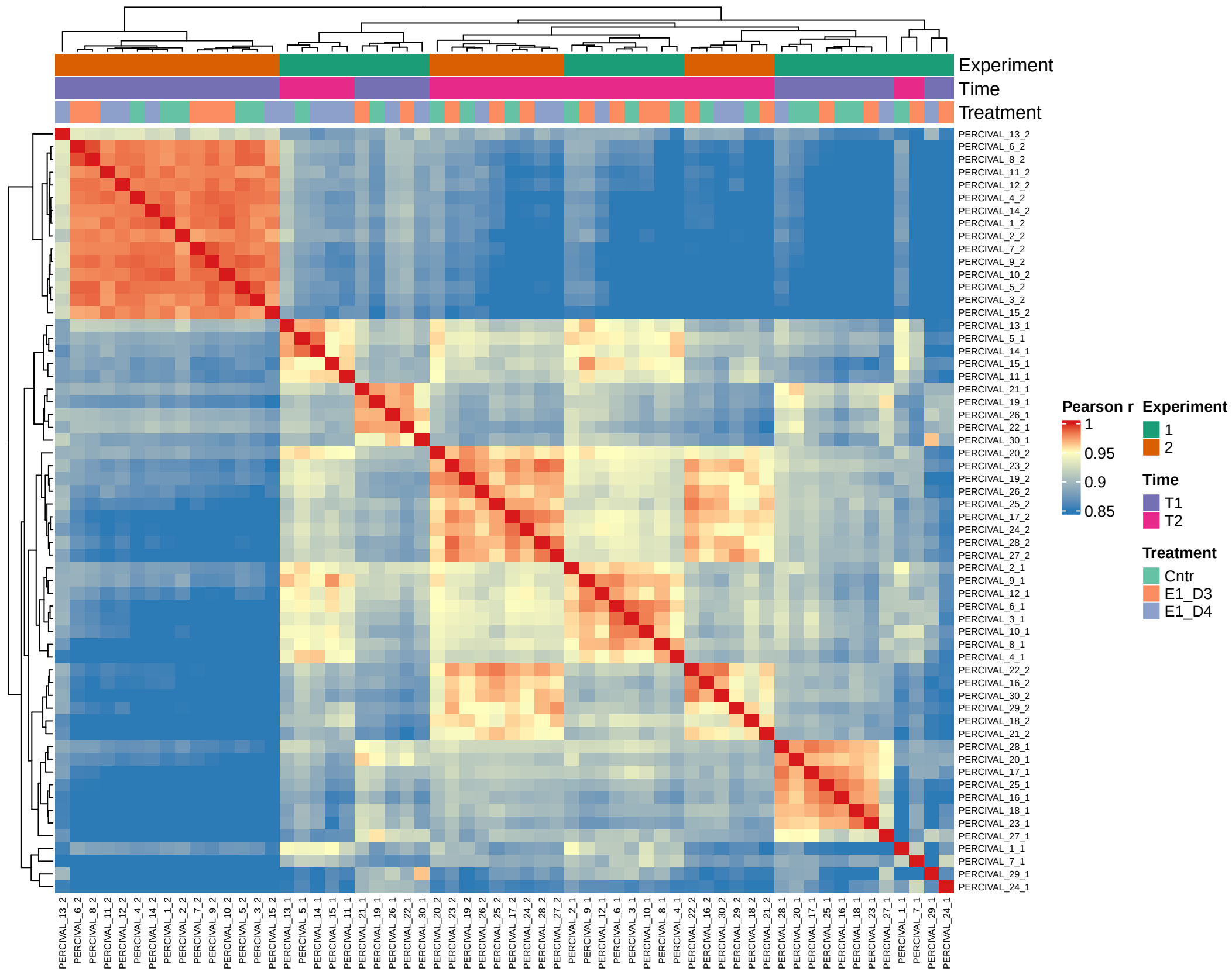
Figure 2C – Pearson correlation (VST counts) of all 60 RNA-seq libraries
