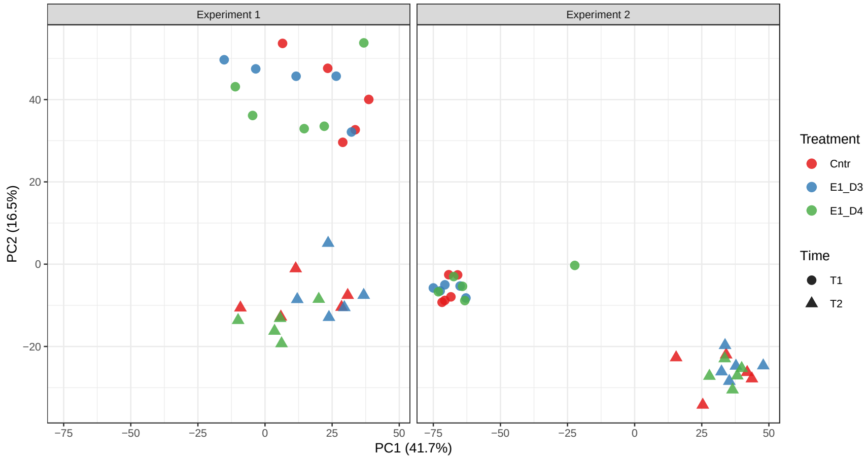
Figure 2D – PCA on top-2000 variable genes (VST)
