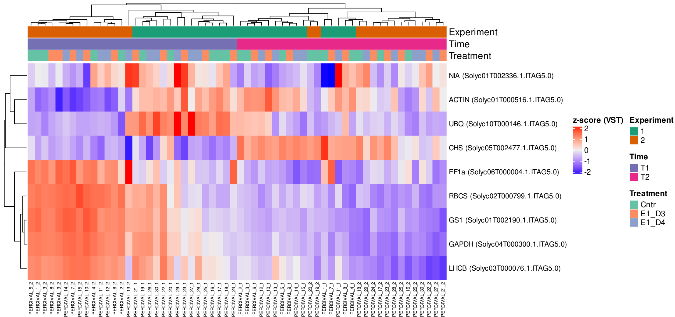
Figure 2E - Marker-gene expression across the 60 RNA-seq libraries (9 markers)
