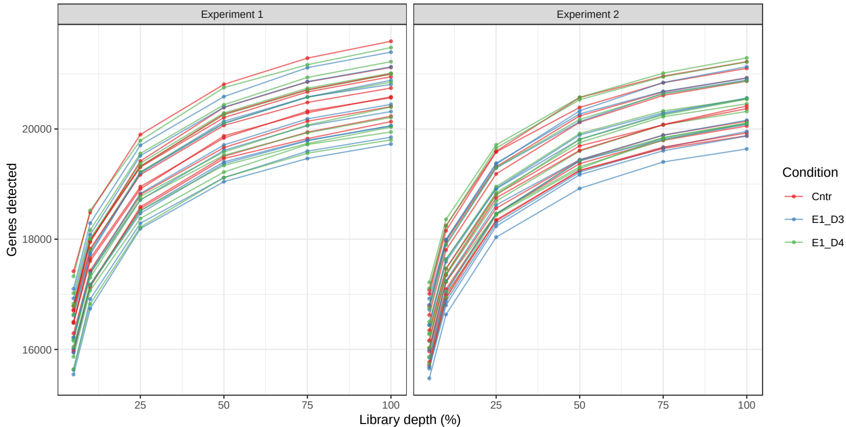
Figure 2F – Gene-detection saturation
