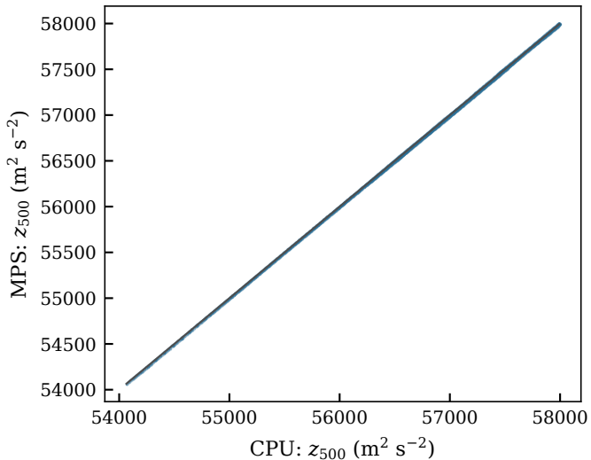
MPS after fix vs CPU r = 1.0000 , \text{RMSE} = 3.9 \text{ m}^2 \text{ s}^{-2}
