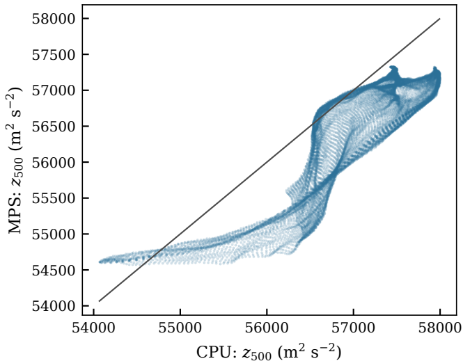
MPS before fix vs CPU r = 0.8721 , \text{RMSE} = 673.1 \text{ m}^2 \text{ s}^{-2}
