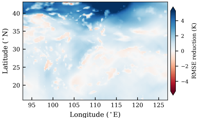
Temperature T @ 850 hPa: error reduction \text{RMSE}(\text{Conv only}) - \text{RMSE}(\text{Conv} + \text{Sat})
