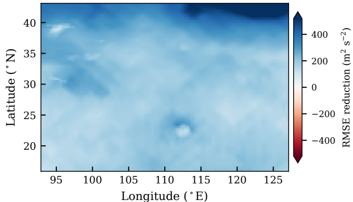
Geopotential z @ 500 hPa: error reduction \text{RMSE}(\text{Conv only}) - \text{RMSE}(\text{Conv} + \text{Sat})
