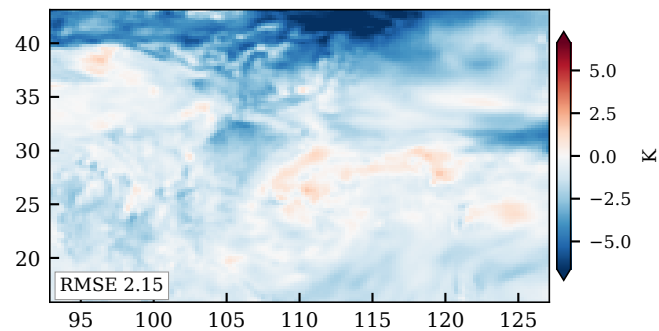
Temperature T @ 850 hPa
