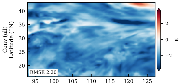
Temperature T @ 300 hPa
