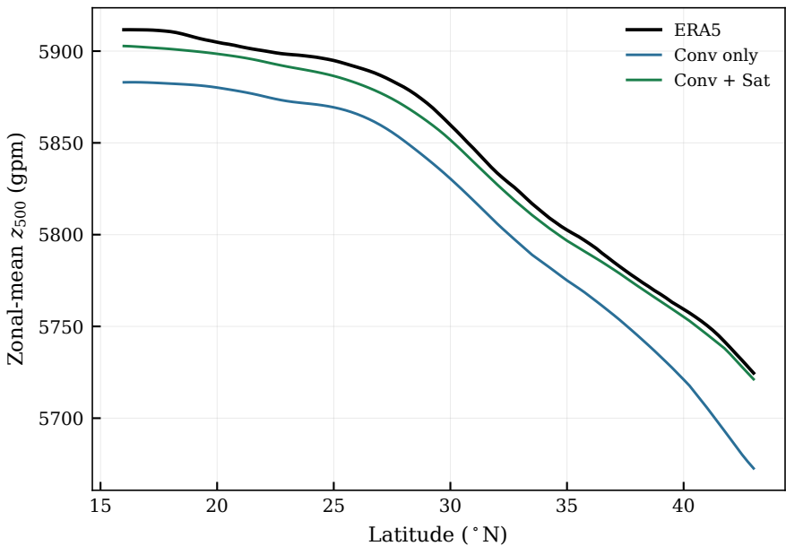
Zonal mean, Geopotential z at 500 hPa
