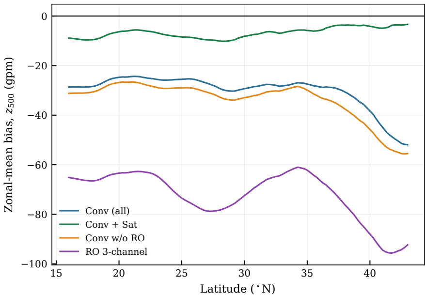
Bias vs ERA5, Geopotential z at 500 hPa
