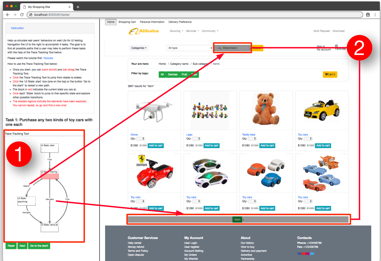
Figure 1. The interactive event-flow graph (①) shows testers’ traces in real time. Testers can go to any previously explored states by clicking the state node. The graph also derives the GUI-level guidance (②) that adds a non-clickable CSS overlay on the previously explored DOM elements to prevent duplicate activity. Currently, this GUI is at the “filtering” event, indicated by the event node with red color in the graph. The red arrows show the overlays are consistent with the outgoing event-flows of the “filtering” event.
