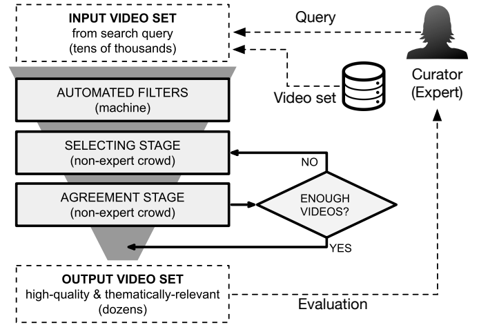
Figure 3: Sifter pipeline.
