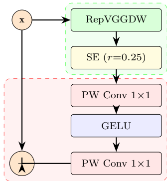
RepViT Block (stride=1)
