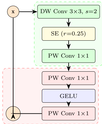
RepViT Block (stride=2)
