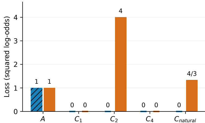
(b) Pairing changes the response penalty
