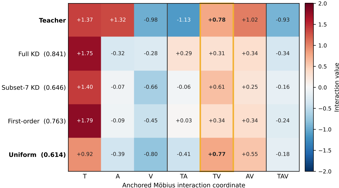
Cross-modal conflict
