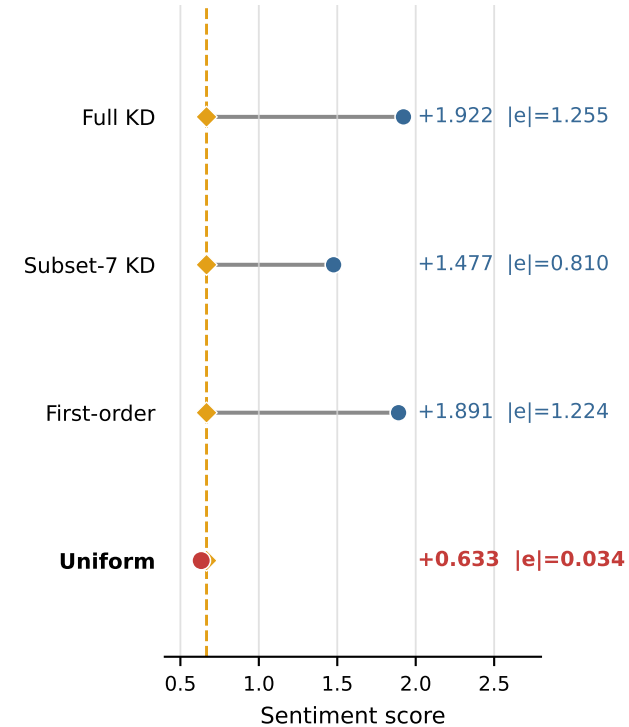
Sentiment prediction Ground truth = +0.667
