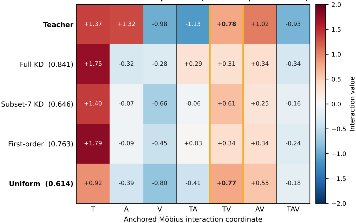
Interaction decomposition (MAE ↓ in parentheses)
