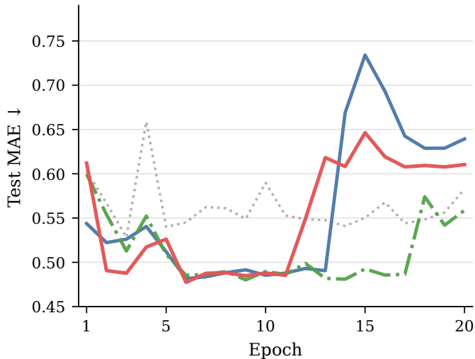
(a) CMU-MOSEI
