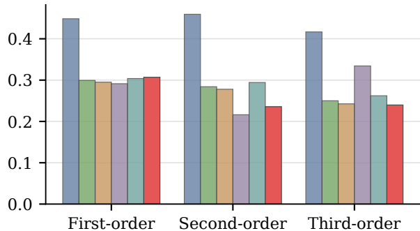
(a) CMU-MOSEI
