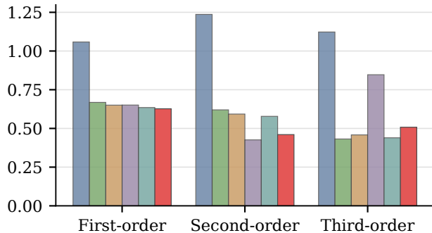
(b) CMU-MOSI
