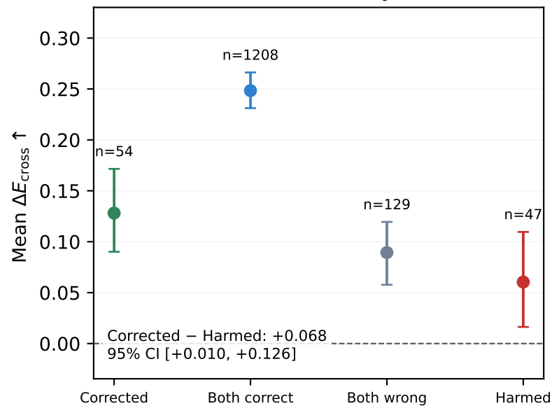
(b) CMU-MOSEI: Polarity outcomes
