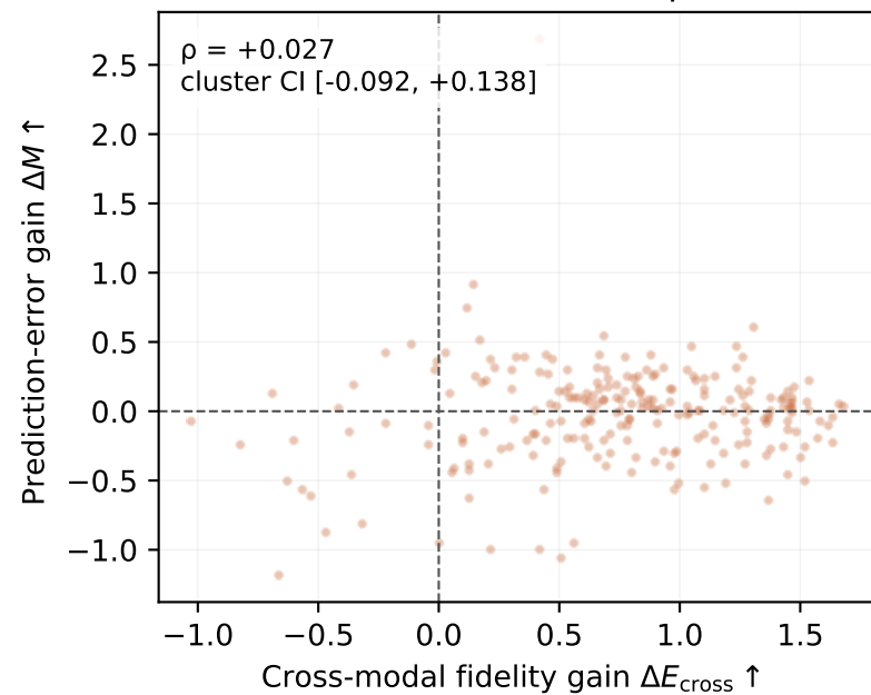
(c) CMU-MOSI: Continuous prediction
