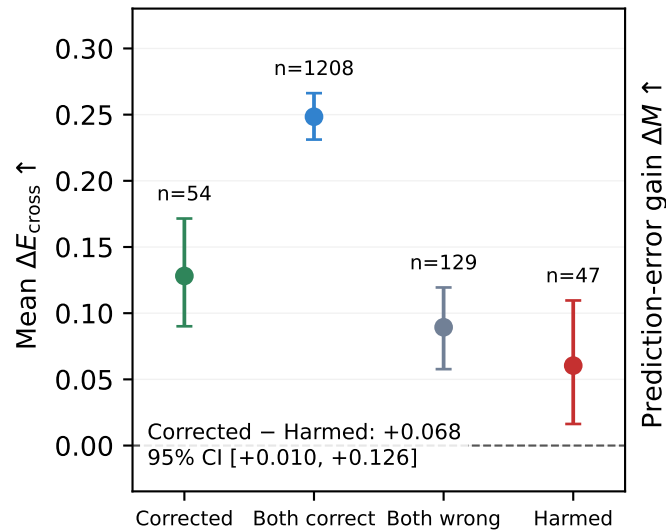
(b) CMU-MOSEI: Polarity outcomes
