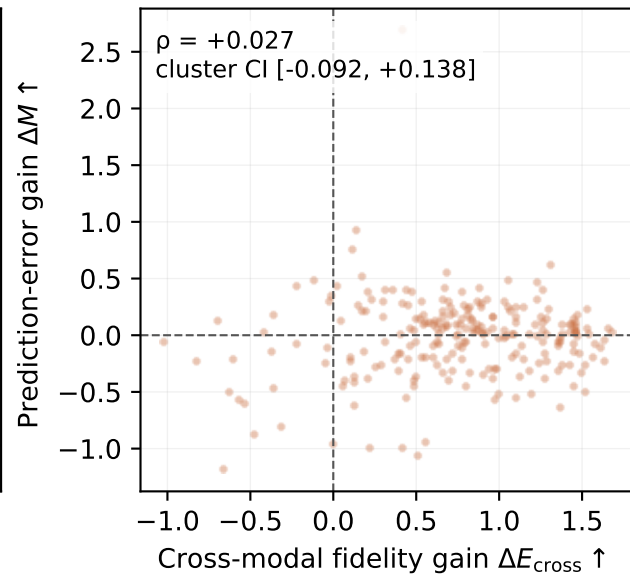
(c) CMU-MOSI: Continuous prediction
