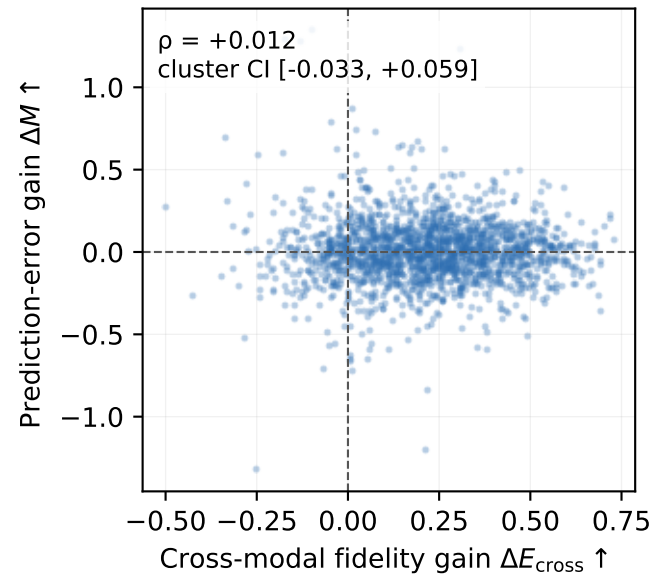
(a) CMU-MOSEI: Continuous prediction
