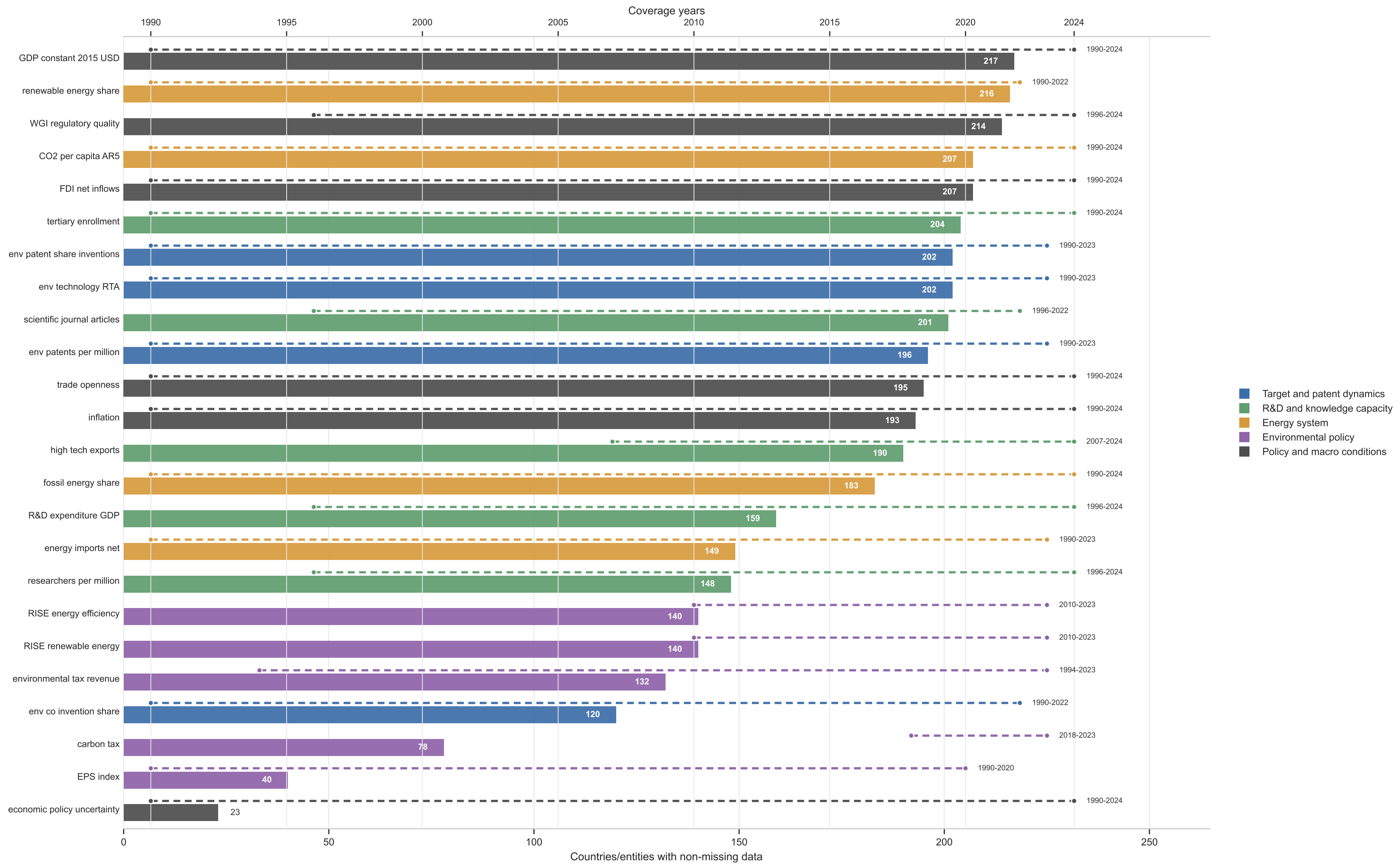
Variable Ranking by Country Coverage and Year Span
