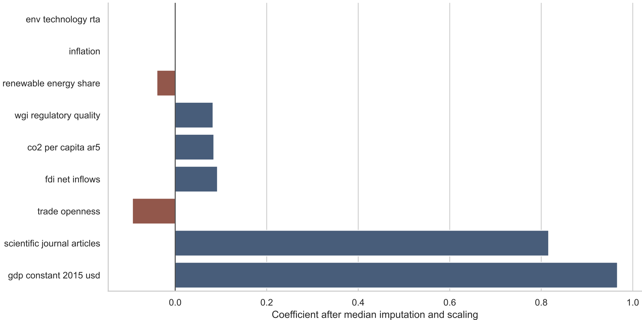
Standardized Linear Coefficients
