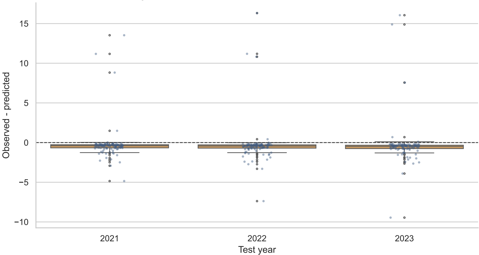
Test Prediction Errors by Year
