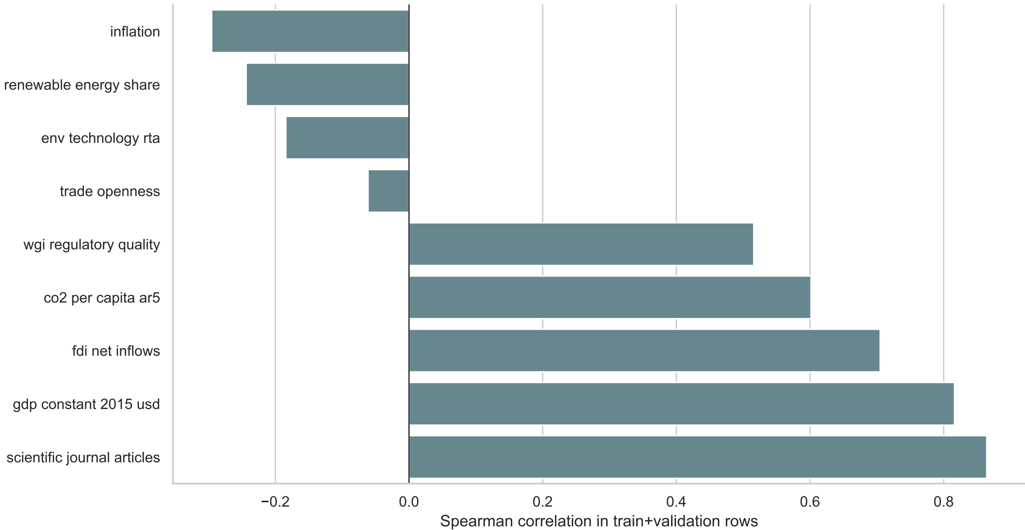
Main Model Predictor-Target Correlations
