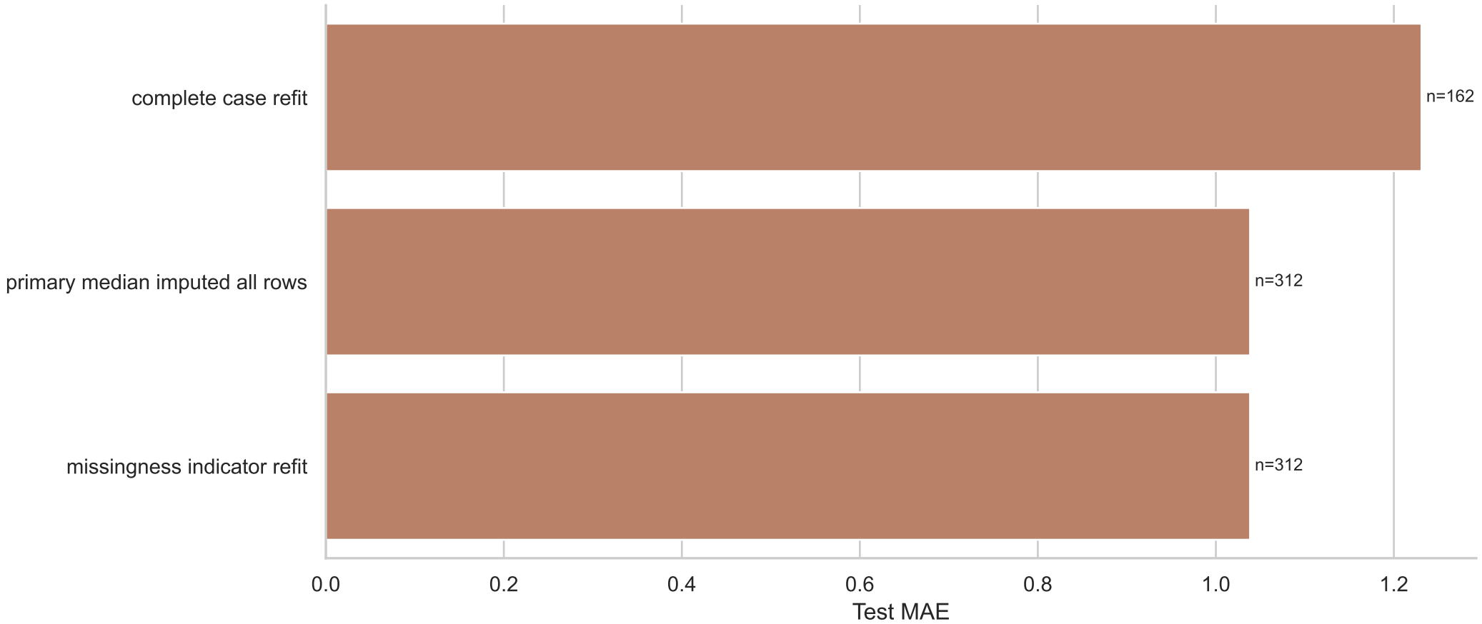
Missingness Sensitivity: Test MAE
