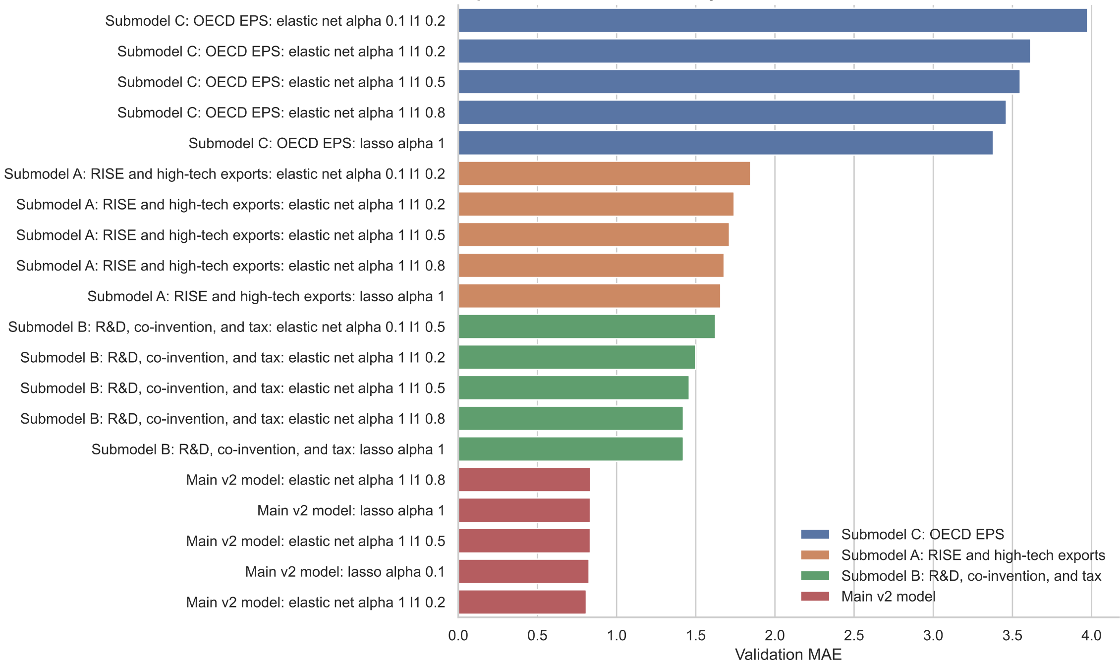
Top Validation MAE Candidates by Panel
