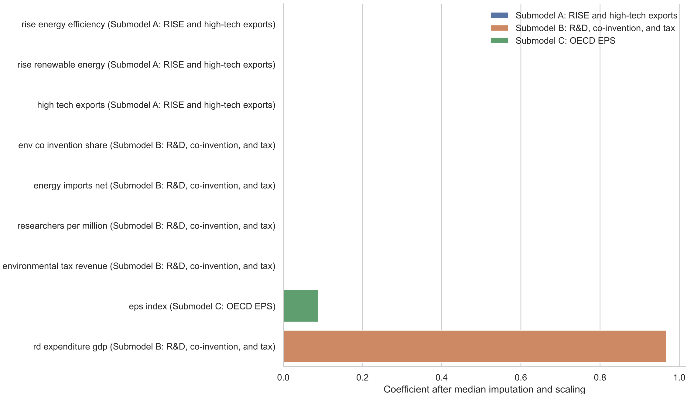
Submodel Standardized Coefficients
