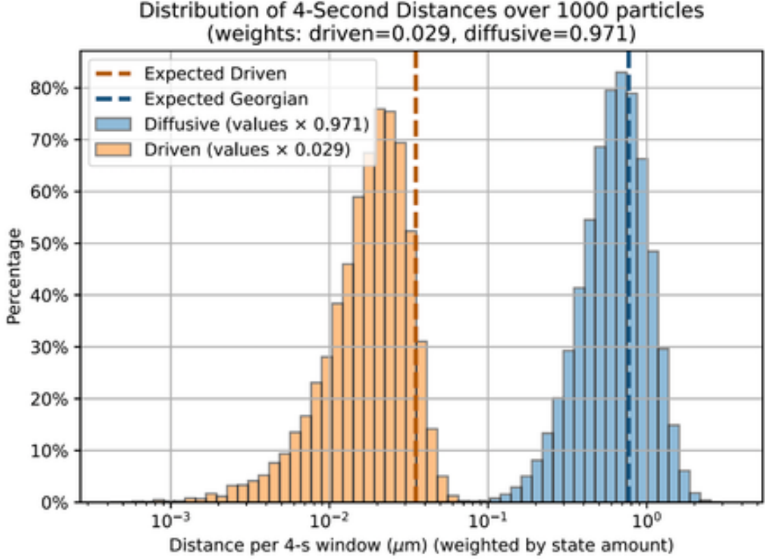
Figure 1: Histogram of “fluxes” over a 4-second window as derived from our simulation. As in the experimental data, motor-enhanced random motion contributes about 20 times as much to the overall particle displacement as driven motion does ( 0.692 \mu\text{m} vs. 0.020 \mu\text{m} ). The blue and orange dashed lines indicate experimental values for distances for motor-enhanced random motion and driven motion respectively, as found in (Holzwarth et al. 2020) ( 0.77\mu\text{m} and 0.035\mu\text{m} ).
