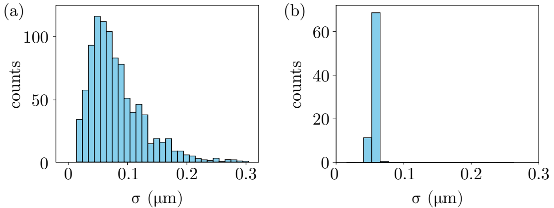
Figure 1.2: The Georgian trap sizes generated by the simulation (subfigure (b)) follow a much narrower distribution as those determined experimentally (subfigure (a)), but with comparable mean: 0.0562 \mu\text{m} , as opposed the experimental value of 0.0825 \mu\text{m} . (Subfigure (a) taken again from (Holzwarth et al. 2020)).
