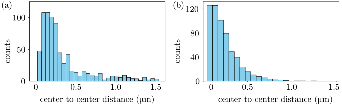
Figure 1.1: The simulated distance between Georgian motion traps (“center-to-center distance”, subfigure (b)) is very similar to the experimentally determined displacement (subfigure (a)). The simulation has a mean trap distance of 0.236 \mu\text{m} , while the experimental data peaks around that value as well (Subfigure (a) taken from (Holzwarth et al. 2020)).
