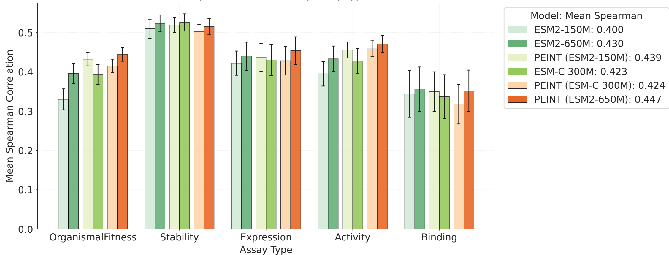
Mean Spearman Correlation by Assay Type
