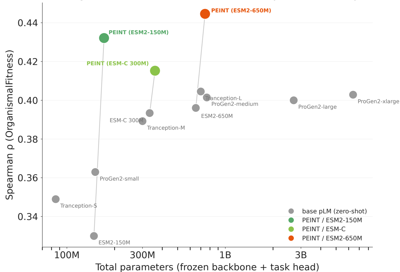
VEP OrganismalFitness vs model size — ProteinGym DMS (69 assays)
