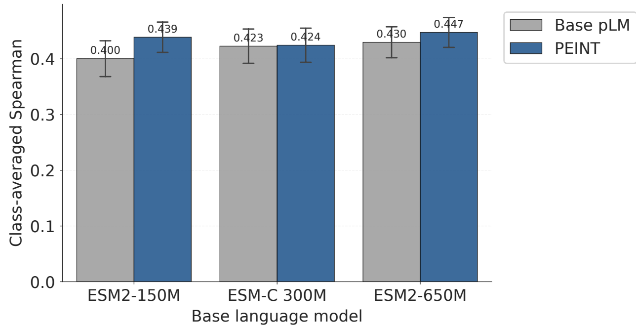
VEP: base pLM vs PEINT by backbone (201 families)
