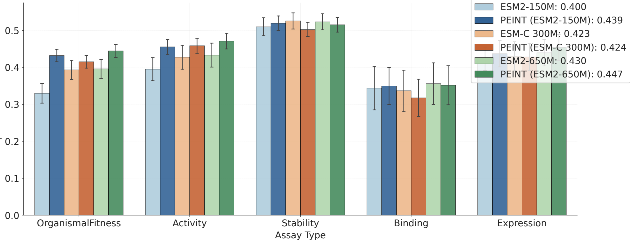
Mean Spearman Correlation by Assay Type
