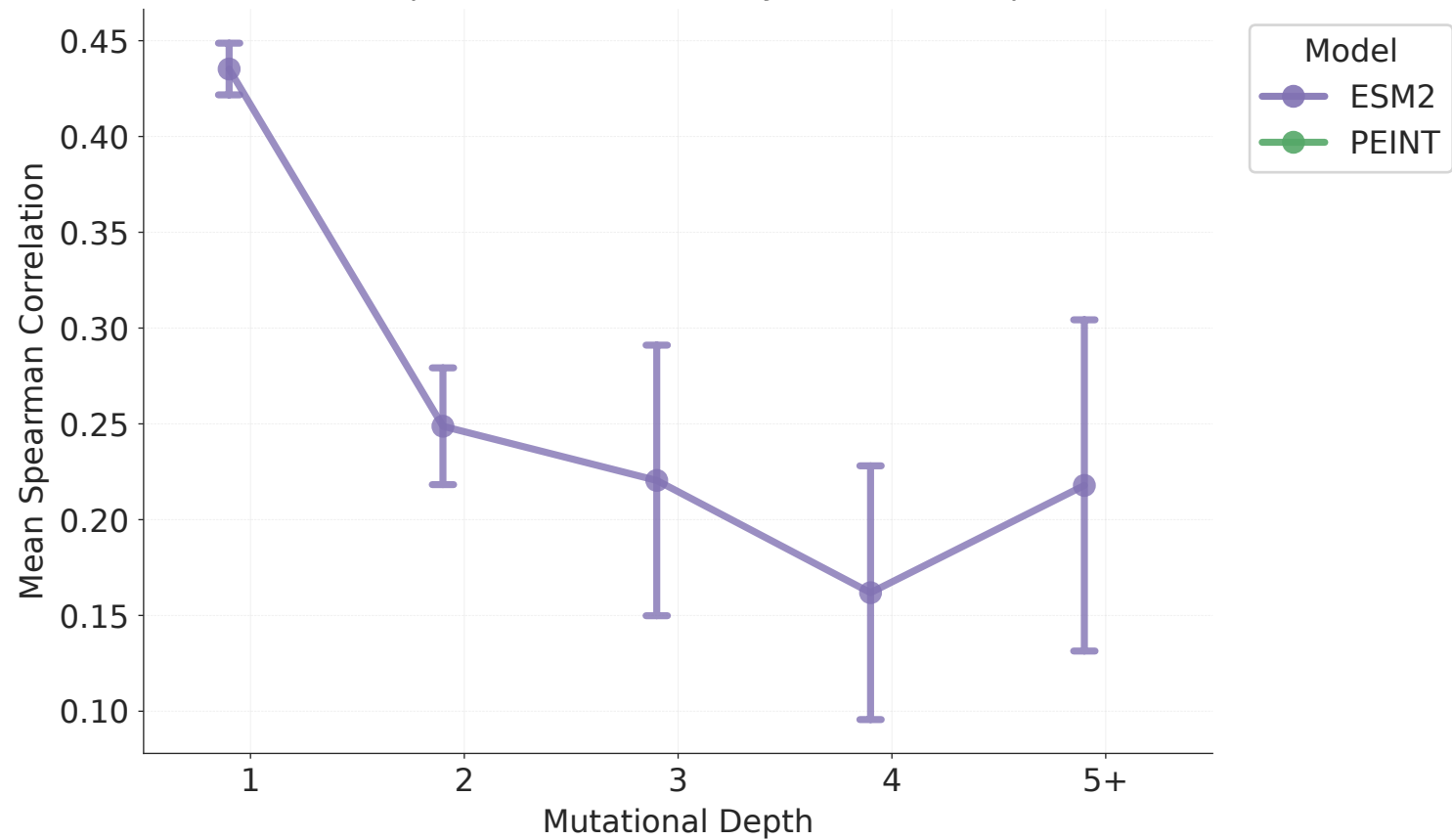
Mean Spearman Correlation by Mutational Depth
