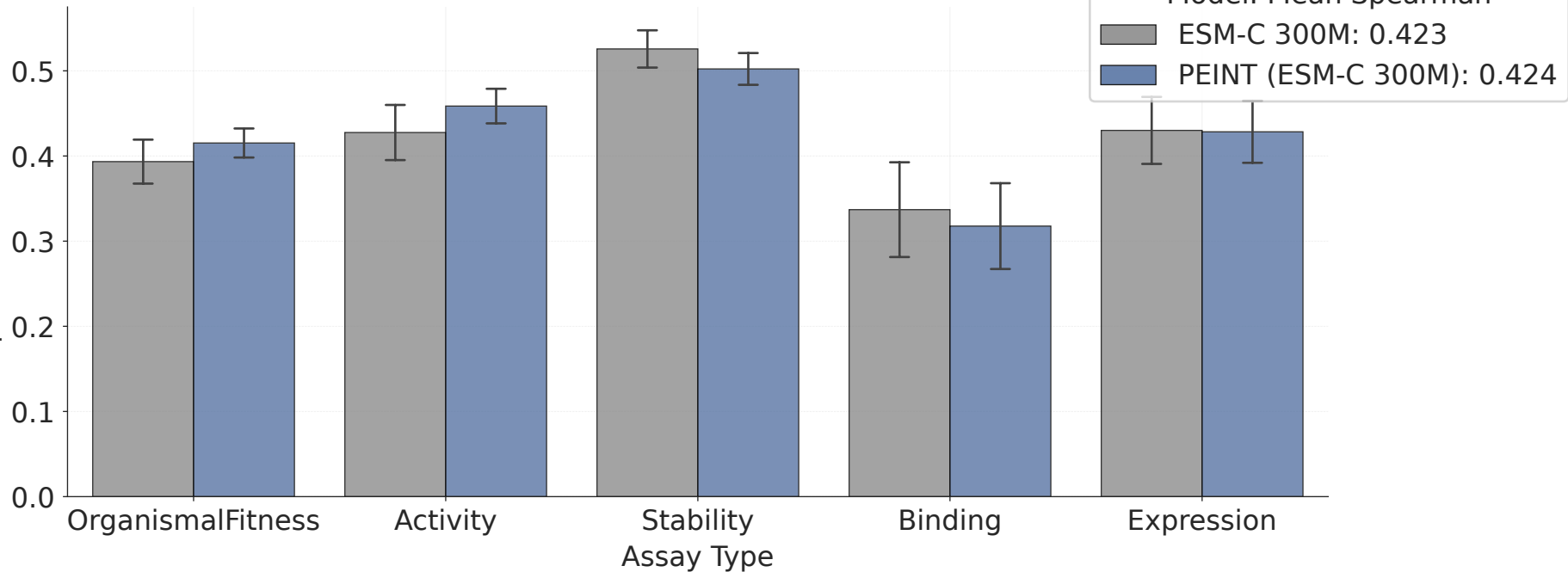
Mean Spearman Correlation by Assay Type
