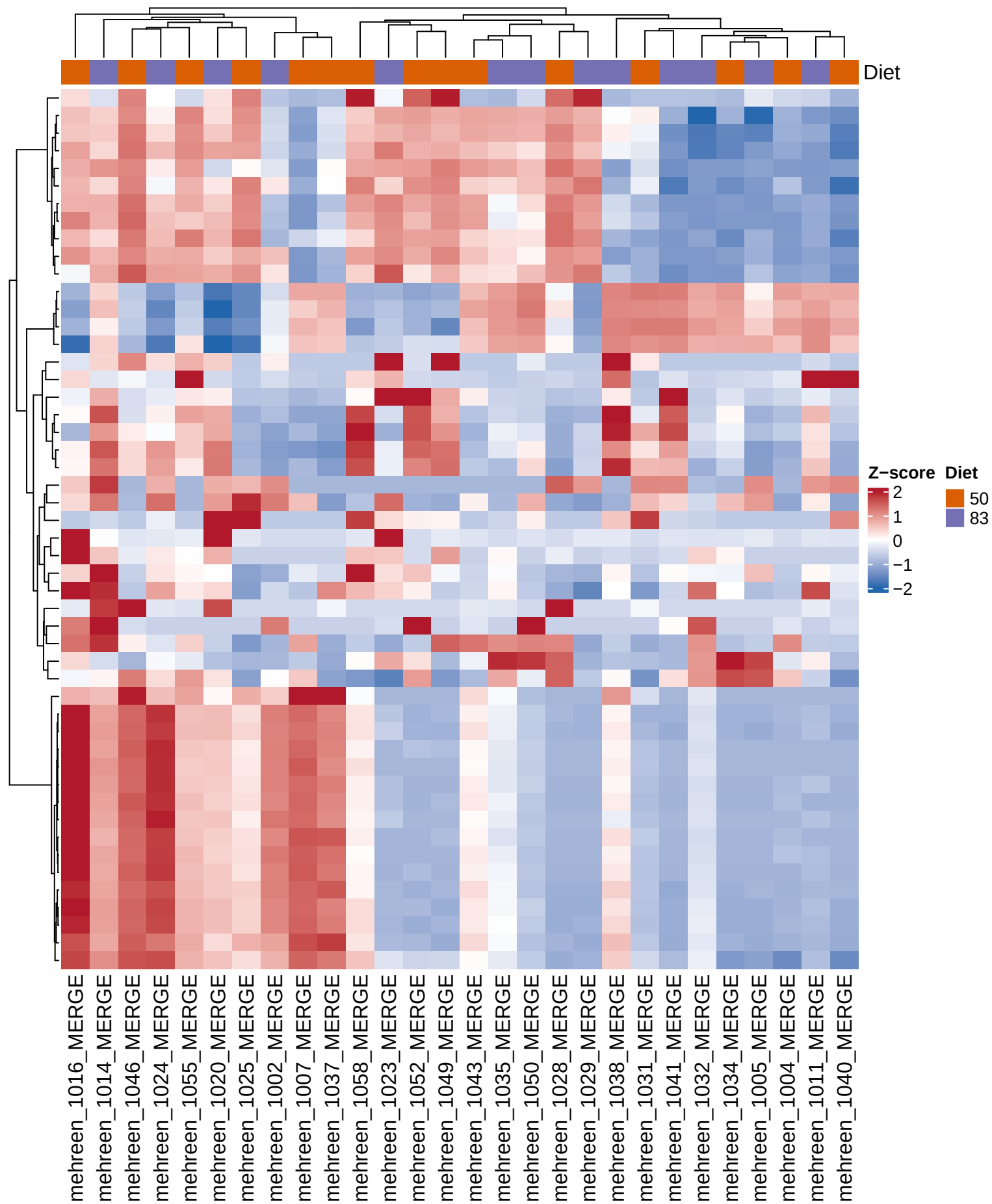
Top Variable Genes: 50 vs 83
