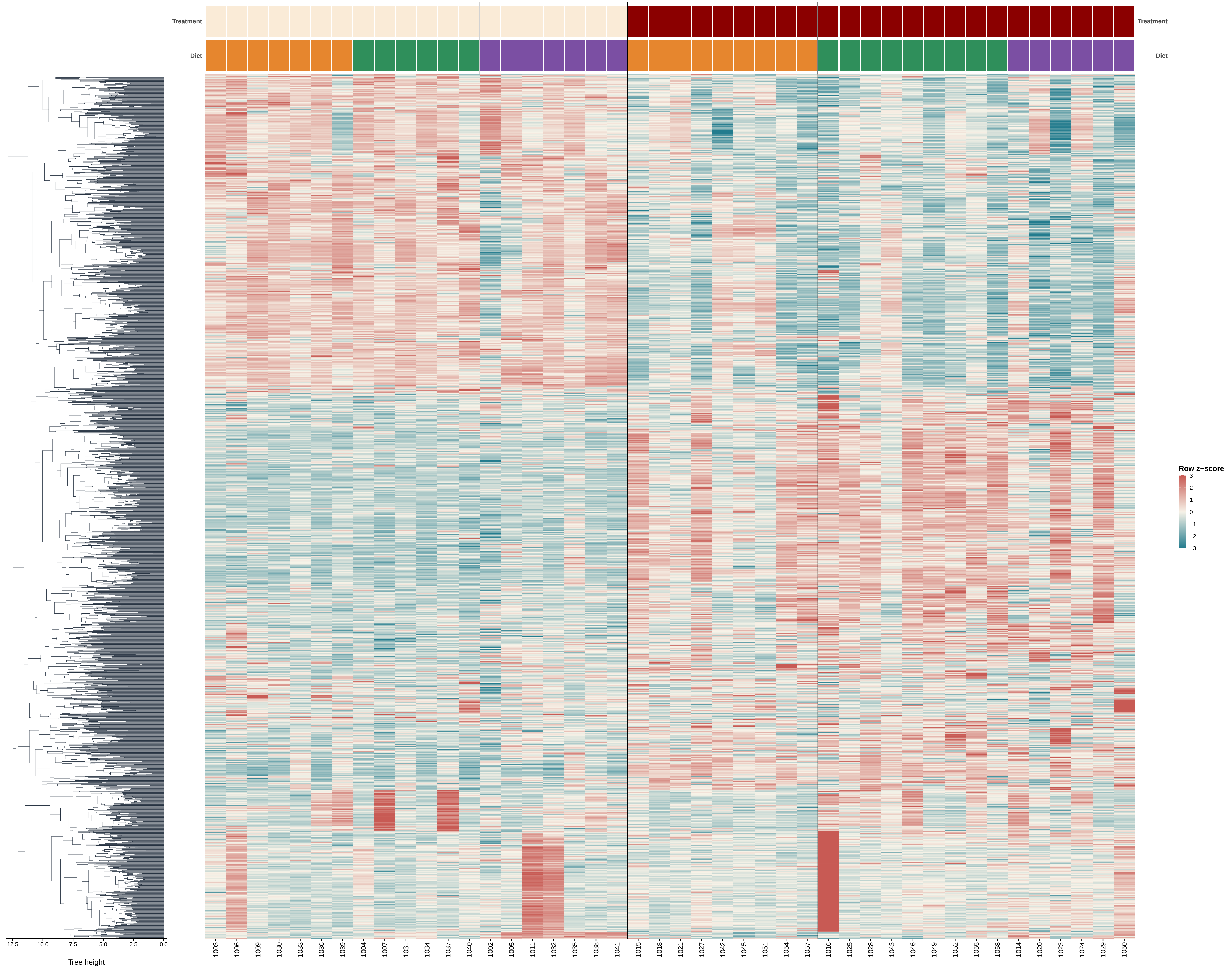
Full main-chromosome DEG heatmap with aligned gene dendrogram (2949 genes)
