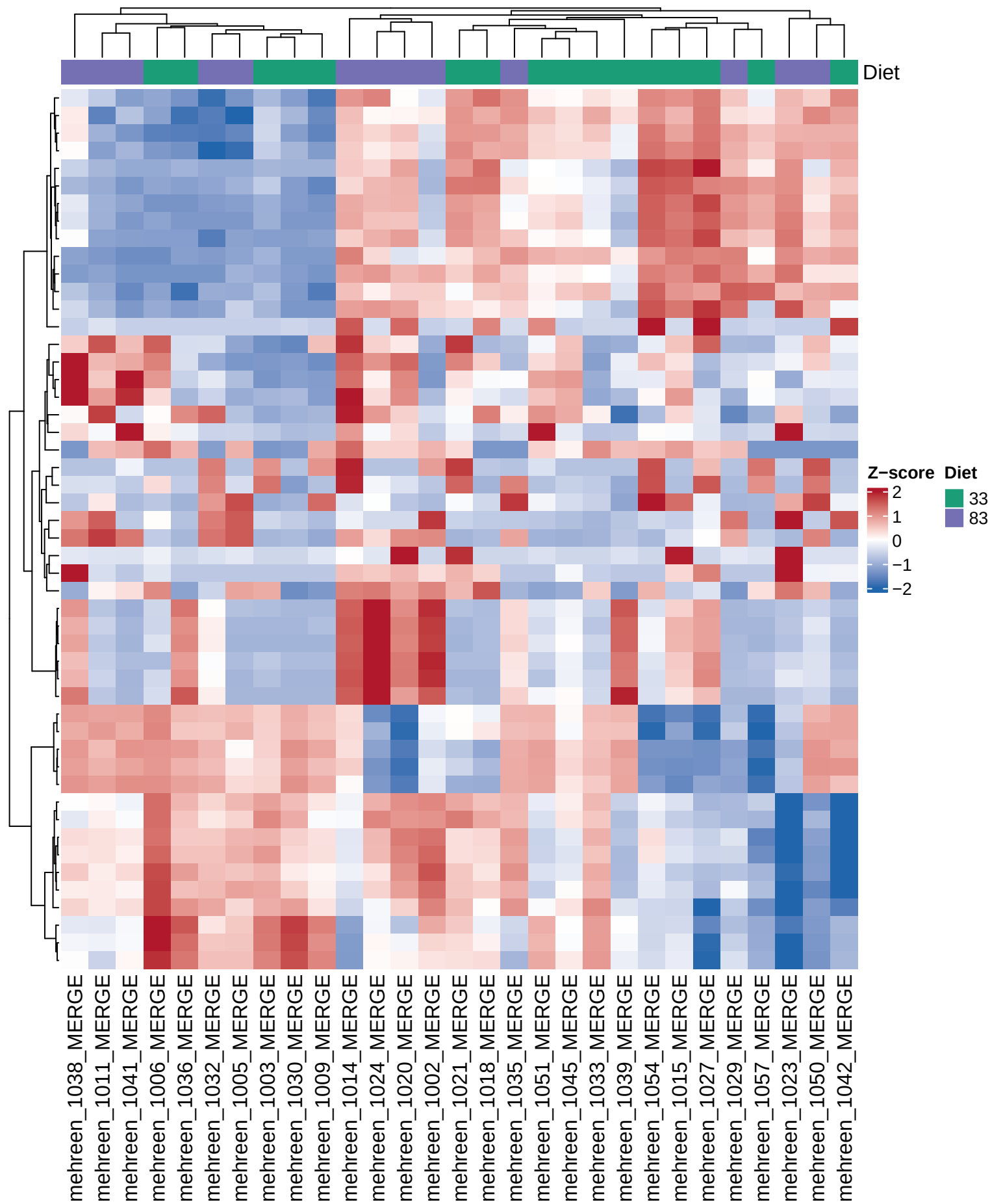
Top Variable Genes: 33 vs 83
