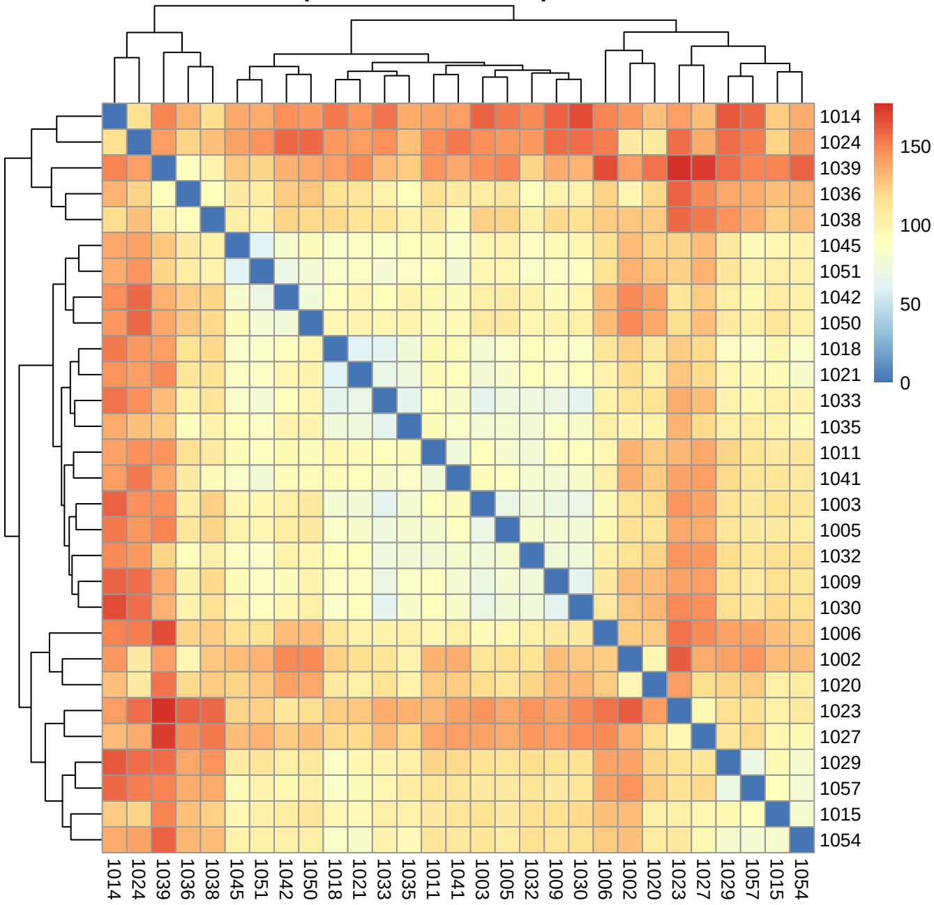
Sample Distance Heatmap: 33 vs 83
