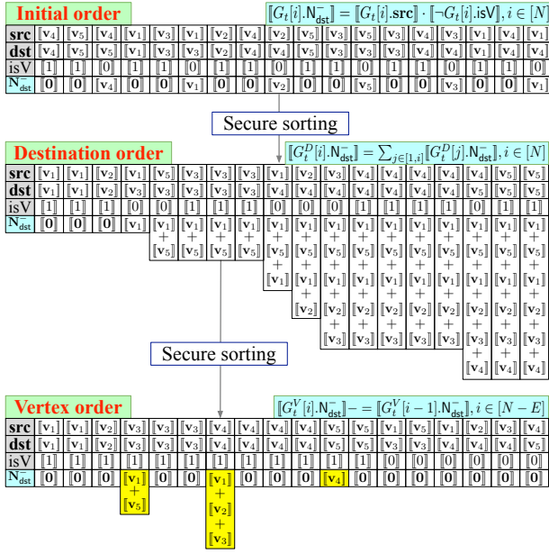
Figure 12: Illustration of secure in-neighbor aggregation on snapshot G_6 in Fig. 2.
