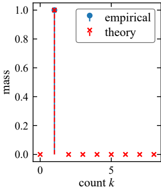
Count PMF (residual)
