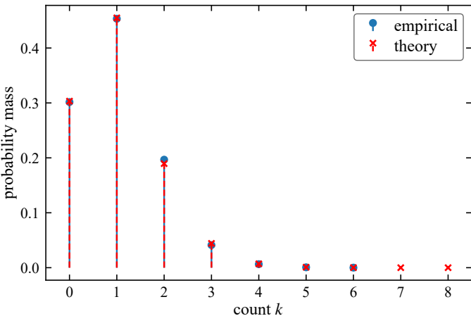
Count PMF (residual) ( N=1000 , d=800 , c=0.8 , n_{\text{rep}}=20 )
