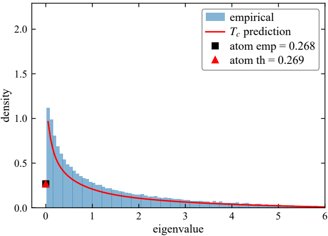
Spectrum (multinomial) ( N=1000 , d=800 , c=0.8 , n_{\text{rep}}=20 )
