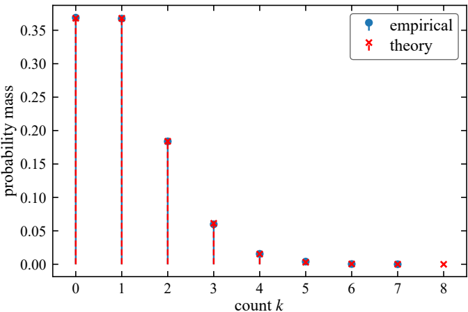
Count PMF (multinomial) ( N = 1000 , d = 800 , c = 0.8 , n_{\text{rep}} = 20 )
