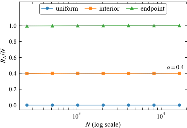
Residual randomization R_N/N
