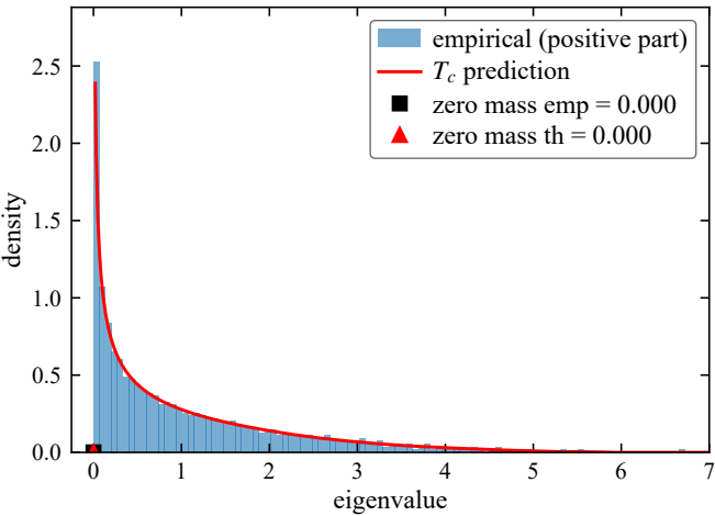
Spectrum: residual, \alpha=0.5 ( N=1024 , c=0.800 )
