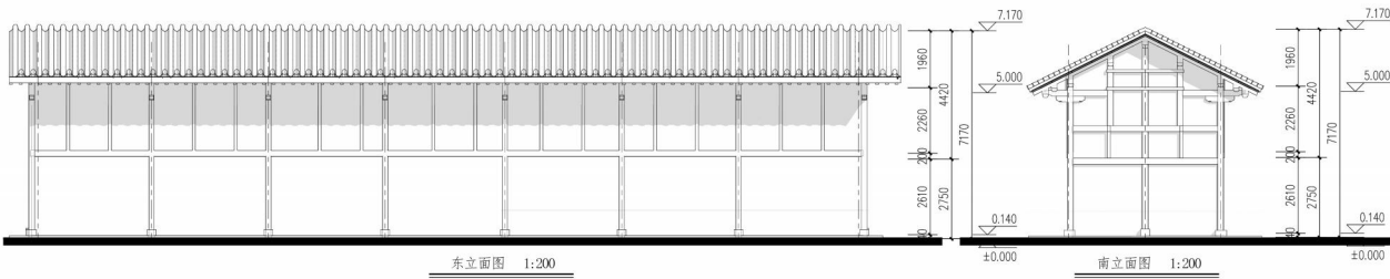
[ 东立面图 ] EAST ELEVATION
