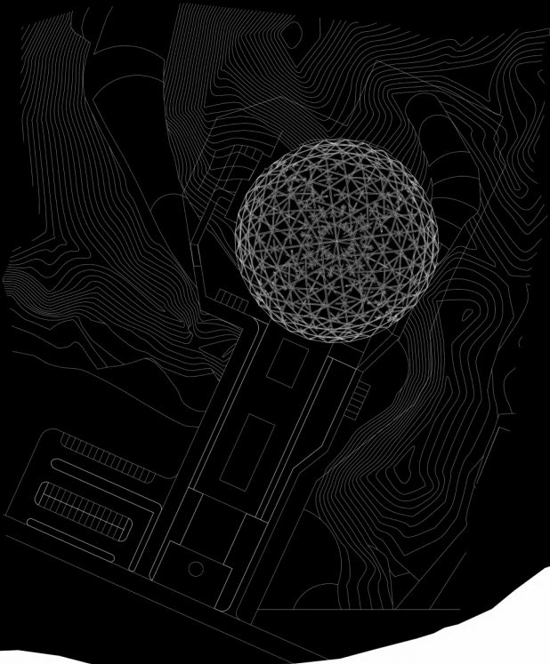
NEGATIVE GROUND FLOOR PLAN 1: 400
