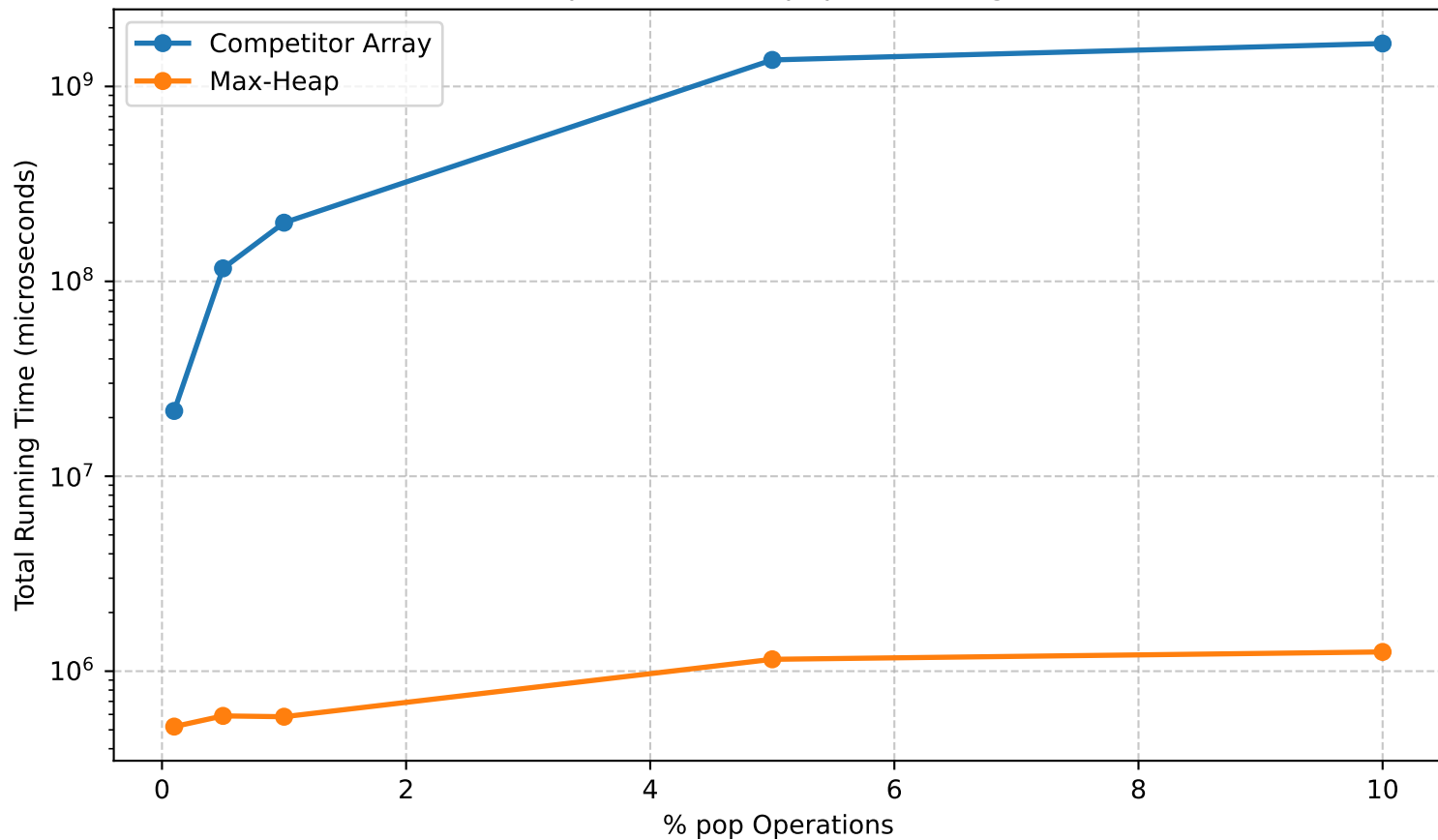
Exp 3: Time v.s. pop Percentage
