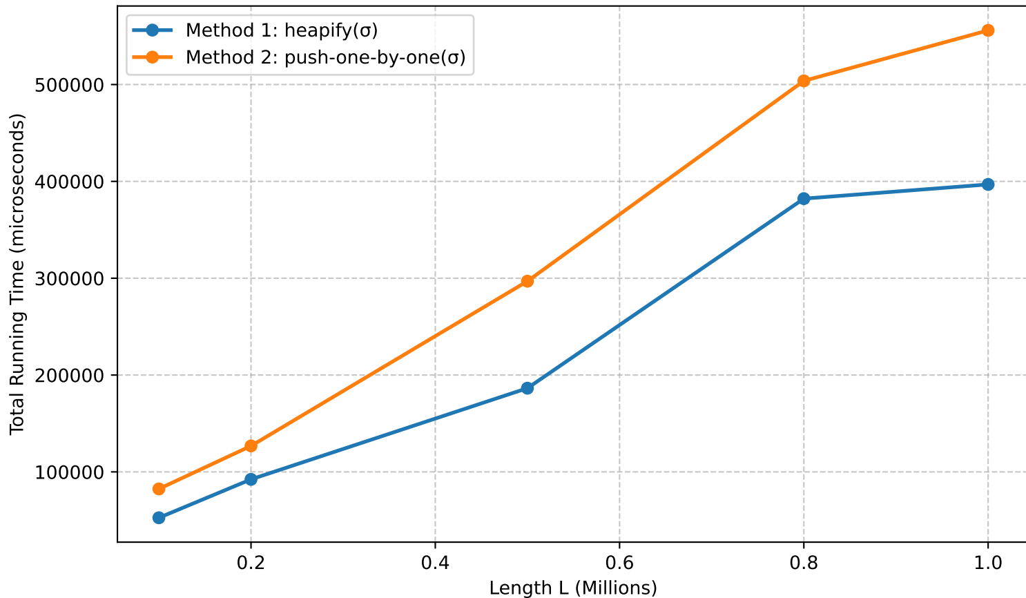
Exp 4: Heapify v.s. Push-One-by-One
