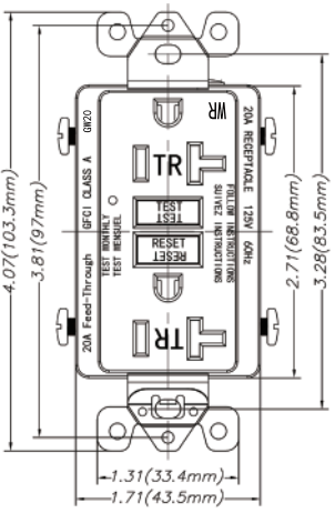
20A Self-Test GFCI
