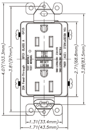
15A Self-Test GFCI
