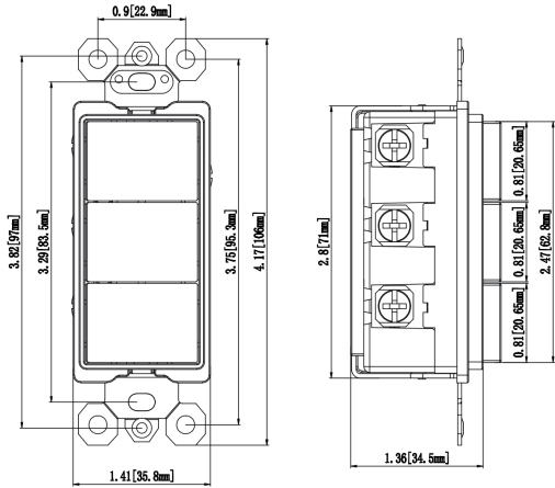
DS1503 Side View
