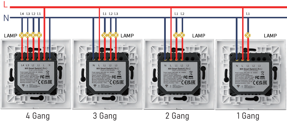
Neutral and Fire Line Wiring Diagram (Neutral Wire Required)
