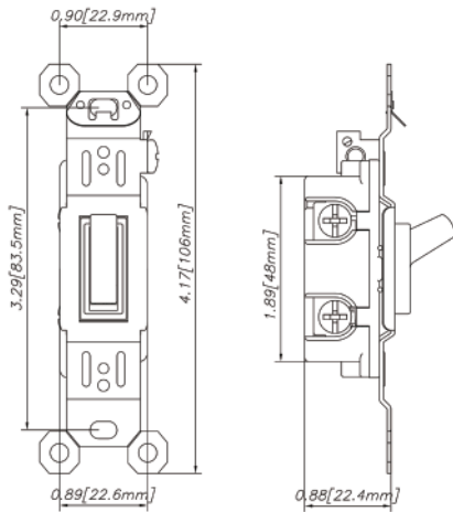
T15 Side View
