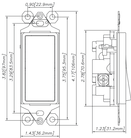
DS15.3 Side View
