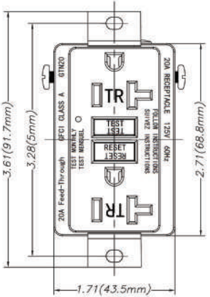
20A Industrial Grade GFCI
