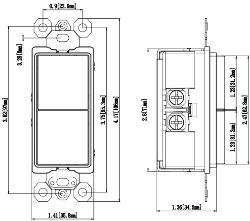
DS1502 Side View
