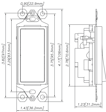
DS15 Side View
