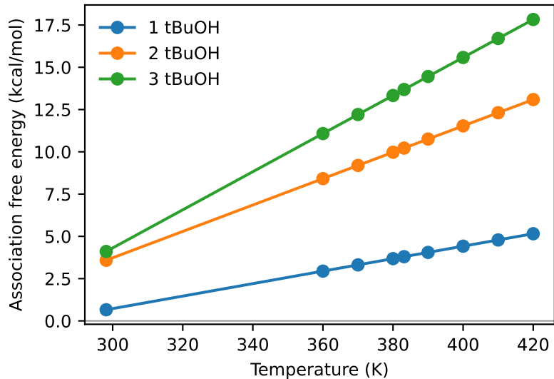
Certified minima; qRRHO, 1 M
