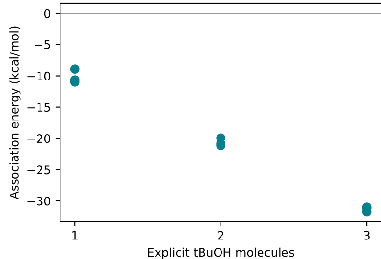
Sampled ALPB model energies
